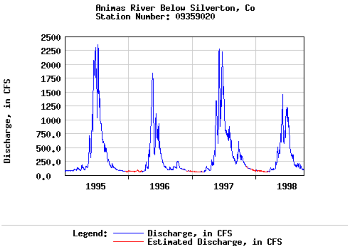
Figure 6. Hydrograph for the period Jan. 1995–Sept. 1998 measured at the USGS gaging station on the Animas River below Silverton, Colorado (A72). Discharge is expressed in cubic feet per second (cfs). Water data are available from http://waterdata.usgs.gov/nwis-w/CO/?statnum=09359020 .
